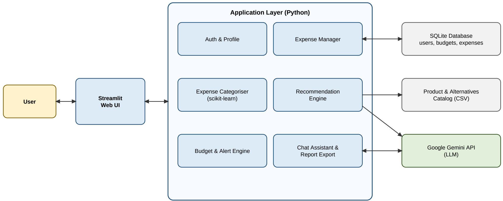
Figure: Solution architecture of PocketSmart AI
